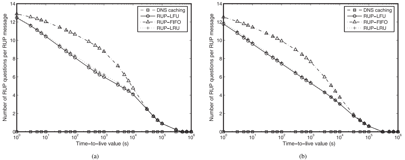
Fig. 9. Average number of RUP questions per RUP message as a function of TTL value: (a) KAIST DNS trace and (b) Yonsei university DNS trace.
